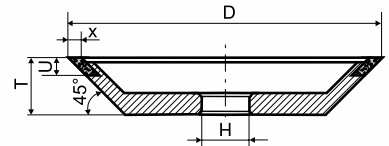
12V9-45° D*U*X*T*H
